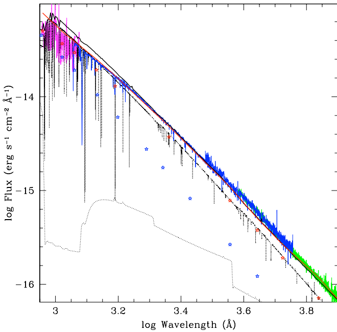
Figure 10. Spectrum of TS 01 from the far UV to the near IR. The observational data after extinction correction and nebular emission lines removal are denoted as follows: FUSE : magenta; HST (FUV+NUV+UVopt): blue; SDSS: green. The models for the nebular and stellar emission are shown by gray dotted lines. The thick black line is the sum of the model continuum emission from the nebular and stellar components. The blackbody solutions are presented by red open stars for the cool component and by blue stars for the hot component. The thick red line is sum of hot (162 kK) and cool ( \sim 57 kK) blackbodies plus nebular emission.
