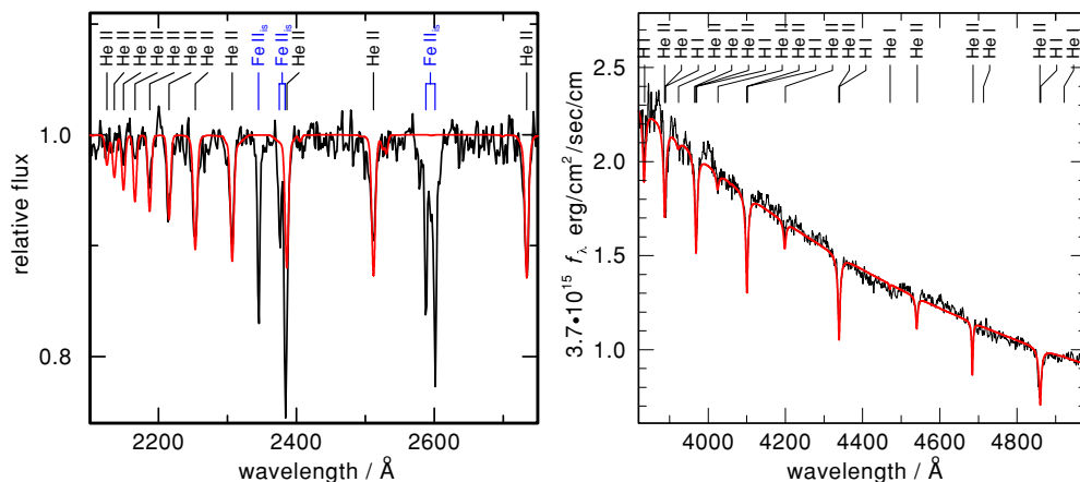
Figure 9. Comparison of a TMAP SED with observation. (a) the STIS NUV range. The He II Fowler series (marked at top) are well reproduced; “is” denotes interstellar lines. (b) the Gemini-North optical range. The H and He lines are marked at top.
