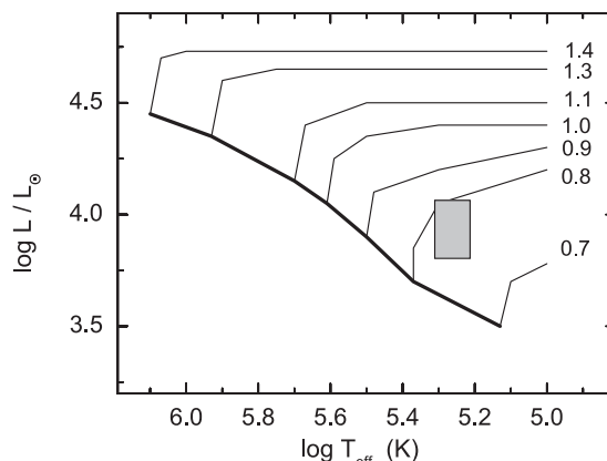
Figure 14. Position of the hot component in the temperature–luminosity diagram (filled box) respective to the tracks of hot accreting WDs in the steady-burning approximation (Iben 1982). The bold solid curve shows the high-temperature boundary of the stable-burning strip. The numbers by the tracks are corresponding WD masses in M_{\odot} .
