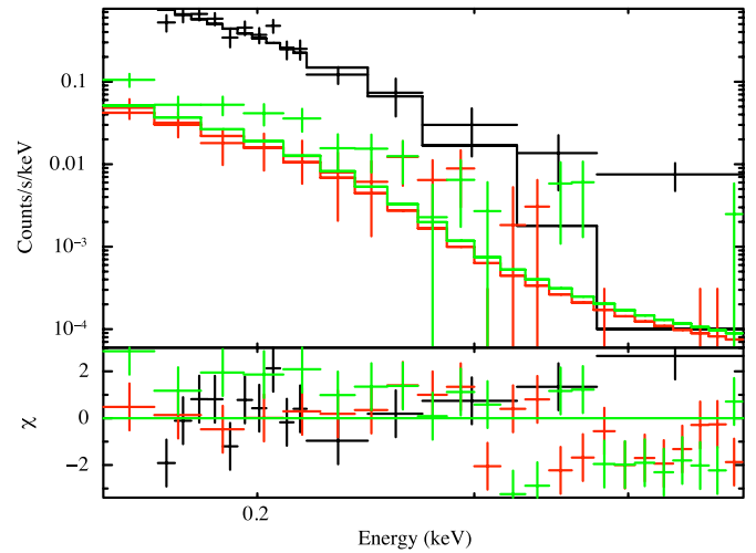
Figure 2. Source spectrum in all three detectors, PN, MOS1, and MOS2 (black, red and green crosses, respectively) are fitted with the same blackbody model (lines of corresponding colors). The photons are concentrated in the lowest 0.1–0.3 keV range. There is general consistency between all three EPIC detectors at energies below 300 eV. In the 0.4–0.5 keV bin, the counts start to differ, but the statistical significance of this is very low taking into account low count rates and calibration uncertainties.
