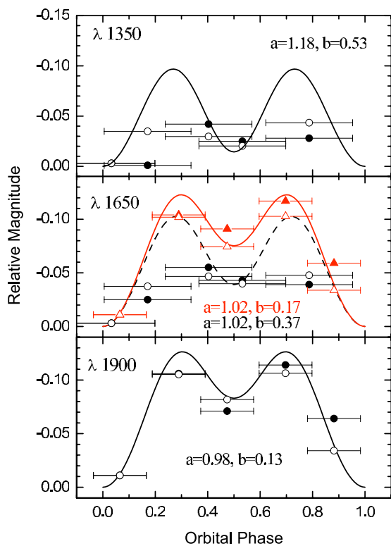
Figure 12. Comparison of the observed light curves (filled symbols) at 1350 Å (top panel), 1650 Å (middle panel), and 1900 Å (bottom panel) with the computed light curves in the same bands (solid and dashed lines). The horizontal error bars mark exposure length for each point. The light curves at 1650 Å are obtained separately from HST FUV (circles) and NUV (triangles) detectors. Their disparity indicates the difference of light curve smoothing due to the exposure length. The model fluxes, integrated in the same phase ranges as observed ones are shown by open symbols. All models are computed for the cool solution from Table 2. To account for differences between the blackbody and real atmosphere we introduced the parameters a and b (see the text), obtained empirically from comparison of these two observed light curves. The values of parameters for flux correction in corresponding bands are marked in the plot. (A color version of this figure is available in the online journal.)
