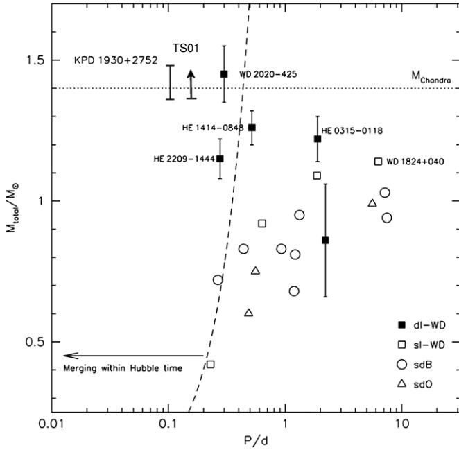
Figure 17. Positions of the known detached double-degenerate systems (DD) and subdwarf+WD systems which will turn into double degenerates. d1: DD with two visible spectra, s1: DD with one visible spectrum. Updated figure from Geier et al. (2007). The position of TS 01 is marked by an arrow, indicating the tendency of better fit to the observed data with increase of total mass of the binary. The minimum value M_{\text{tot}} \geq 1.35 M_{\odot} corresponds to the leveling of \chi^2 slope in Figure 13. We consider the values at plateau in the \chi^2 - M_{\text{tot}} dependence as a range of best solutions.
