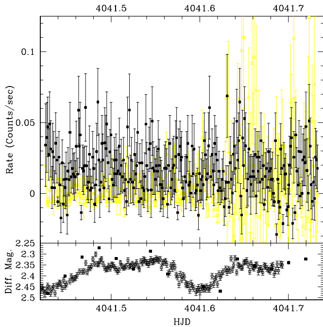
Figure 3. X-ray light curve of the source in the PN detector (top panel). The filled symbols represent the light curve in the 0.1–0.3 keV range, while the open symbols (yellow) are the counts in the 0.3–10.0 keV band. The count rate above 0.3 keV is practically zero, except during the final part of the exposure, where they are dominated by background flaring. In the extreme soft band, 0.1–0.3 keV, the count rate is approximately constant ( 0.033 \text{ counts s}^{-1} ) for the entire duration of the observation. The bottom panel displays the optical light curve for comparison. Black points are OM measurements on board of XMM-Newton at the time of the observations whereas the open boxes are V light curve obtained at SPM (2.5 yr earlier; shifted in time according to phases). (A color version of this figure is available in the online journal.)
