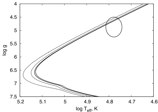
Figure 8. T_{\text{eff}}\text{-log } g dependence for post-AGB models (Weiss & Ferguson 2009 and A. Weiss & J. W. Ferguson 2009, private communication). Solid line: Z = 0.004 for 0.529 and 0.533 M_{\odot} . Dashed line: Z = 0.0005 for 0.539 and 0.551 M_{\odot} correspondingly. Tracks for more massive stars spread out toward hotter temperatures. The ellipse indicates the range of possible solutions for TS 01 stemming from a variety of methods used in this paper.
