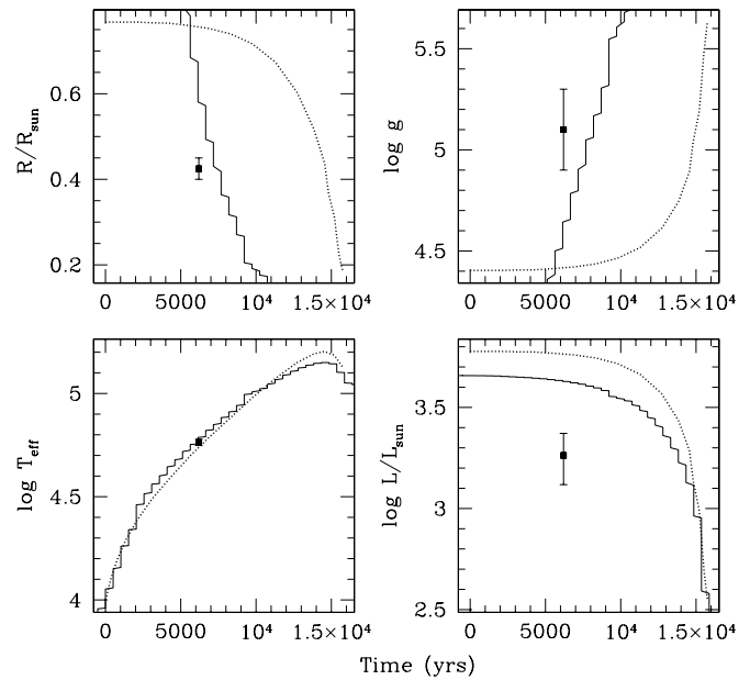
Figure 16. Various parameters of the models of post-AGB stars vs. time. Solid line is for the M = 0.547 M_{\odot} , Z = 0.0005 model Weiss & Ferguson (2009), dotted line is for the M = 0.623 M_{\odot} , Z = 0.001 model Vassiliadis & Wood (1994). TS 01 is marked by squares with error bars at age of ( \sim 6000 yr), appropriate to its effective temperature.
