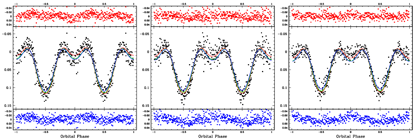
Figure 11. From left to right, the Nightfall fits to the light curves in u , v , and r . In the main panel, the red, green, and blue curves represent the solution for X-component with T_{\text{eff}} of 162 kK, 182 kK, and 202 kK, respectively. The deviations with respect to the coolest and hottest solutions are shown in top and bottom panels, respectively. The complete set of parameters used in fitting is given in Table 3. The simultaneous fit to the RV curve is similar to the sin curve presented in Figure 6.
