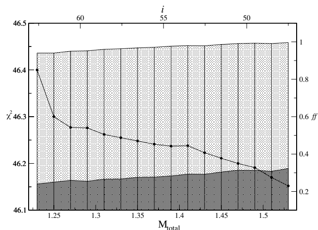
Figure 13. Line with dots depicts the dependence of the \chi^2 value on the total mass of the system. Fixed parameters in the calculations were the temperatures of the components (55 and 160 kK, respectively) and M_{\text{cool}} ( 0.54 M_{\odot} ). The free parameters were the inclination of the binary orbit i , which changed similar to the \chi^2 in a range of values shown on the upper axes; and the Roche lobe-filling factors ( ff ) of both components shown as shaded areas in a range of values marked on the right side axes. The dark shaded area corresponds to Roche lobe-filling factor of the hot component and the light gray to that of the cool component.
