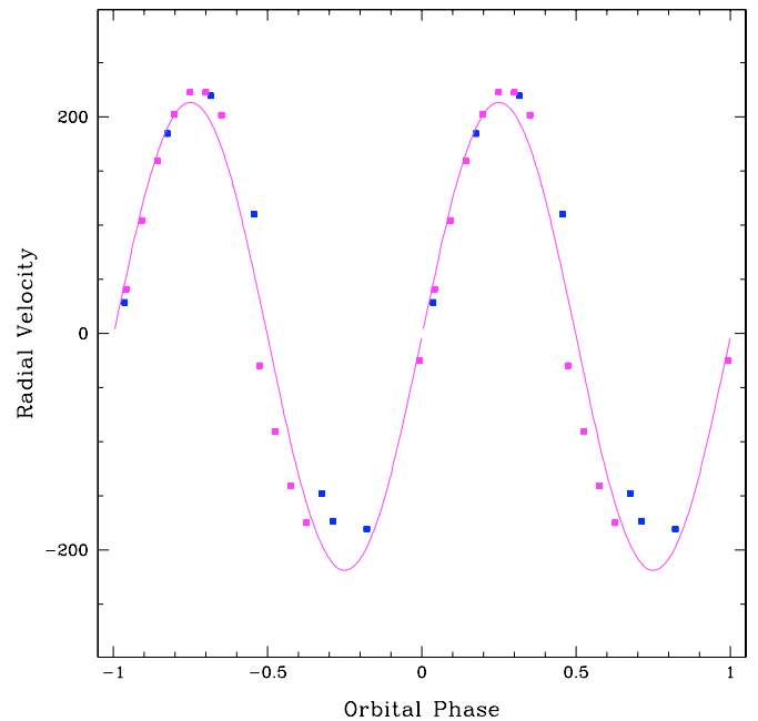
Figure 6. RV curve of TS 01 folded with the orbital period. The points marked in magenta are measurements from Gemini spectra. The CFHT points are presented in blue. The latter were measured anew with the same parameters deduced from the line profile fitting by FITSB2. The sin fit to the data presented here is practically indistinguishable from RV curve calculated by Nightfall (see below).
