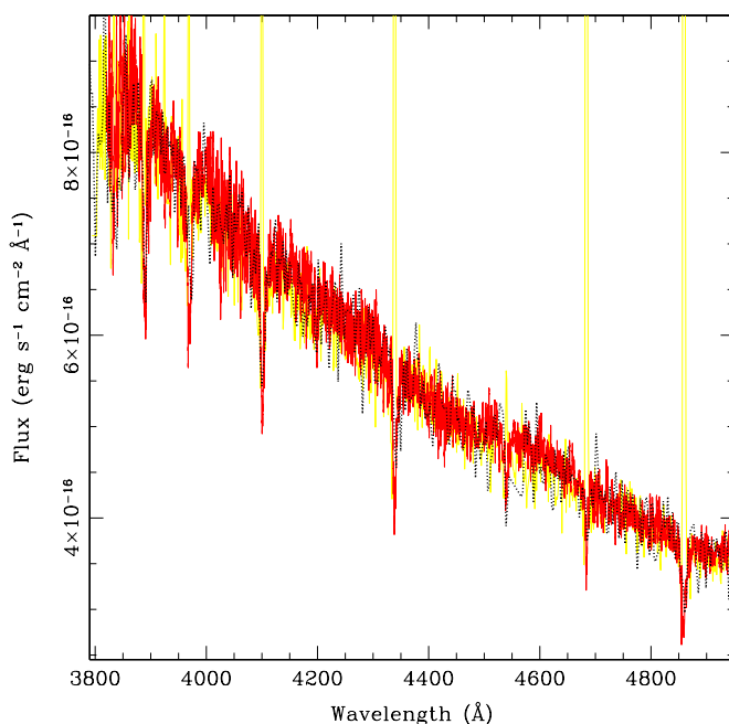
Figure 1. Stellar spectrum of TS 01 obtained at Gemini-North (solid red line). The spectrum is a combination of 12 individual spectra, observed at different orbital phases, and smoothed with a 13 pixel boxcar. Before combining, the individual spectra were corrected for orbital motion. The SDSS spectrum, containing nebular lines, is plotted in yellow. The black dotted line is the single HST spectrum obtained for the same spectral range (see the text). (A color version of this figure is available in the online journal.)
