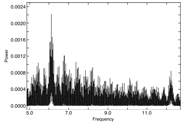
Figure 4. Power spectrum of all photometric data. The strongest, single peaked maximum corresponds to the orbital period, at 6.1159 \text{ day}^{-1} . The first harmonic, at \approx 12 \text{ days}^{-1} , is also prominent in the power spectrum because of the double-humped nature of the light curve.
