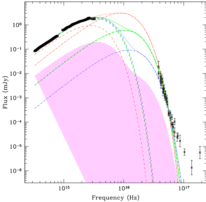
Figure 7. SED of TS 01. The observed spectra are presented by crosses with error bars (SDSS + HST /STIS + FUSE + XMM ). The observations are fitted with two blackbodies. Three pairs of blackbody solutions are presented according to Table 1. Dashed, dash-dotted and dotted lines represent the cool , the hot components, and their sum, respectively. Shaded is the area in which the radius of hot component determined from the light curve analysis starts to deviate from the one required for SED fitting. In this area the luminosity of hot component does not provide enough irradiation to the cool component to produce observed light curve. Thus, only a cool \sim 160,000 K solution is viable.
