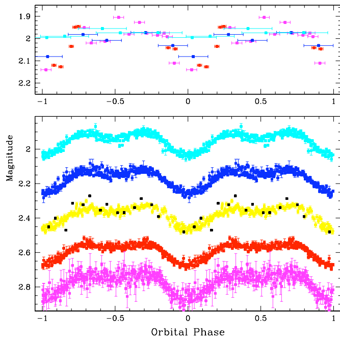
Figure 5. Light curve of TS 01 folded with the orbital period. The lower panel presents optical light curves. From top to bottom are: BUSCA UV and B, Johnson V from SPM, XMM OM (black points), and finally BUSCA R and NIR. The upper panel presents HST data: H_\alpha (red), [Ne v] (magenta), the integrated spectral flux in the NUV (dark blue) and FUV (cyan). The horizontal error bars in the upper panel denote the exposure time converted to orbital phase.
